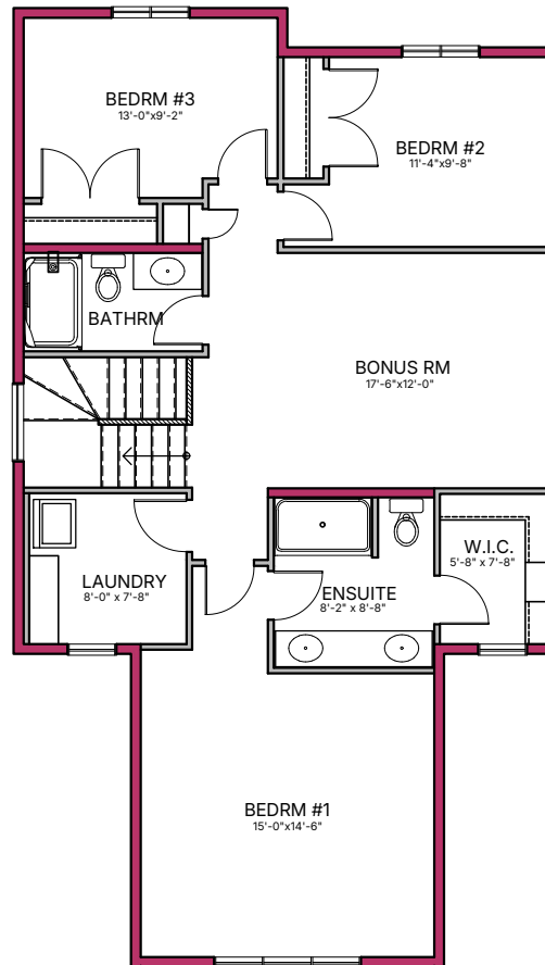
SECOND FLOOR - 1,093 sq.ft. OPEN AREA - 59 sq.ft.
