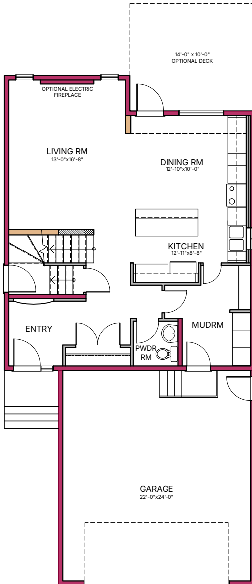
MAIN FLOOR - 868 sq.ft.
