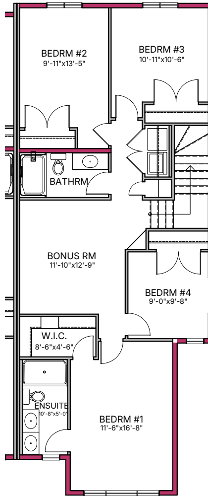
SECOND FLOOR - 1024-1062 sq.ft. OPEN AREA - 50-58 sq.ft.
