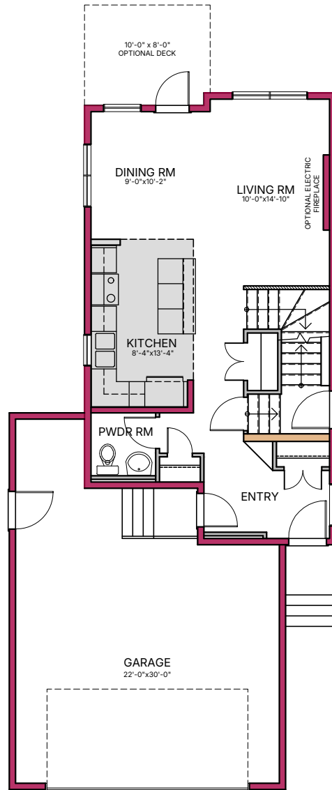
MAIN FLOOR - 670 sq.ft.
