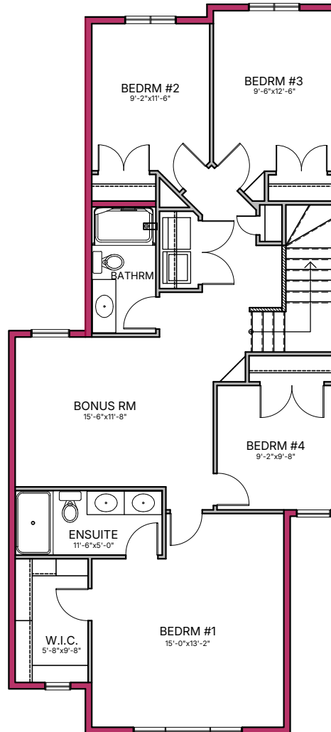
SECOND FLOOR - 1,172 sq.ft. OPEN AREA - 58 sq.ft.
