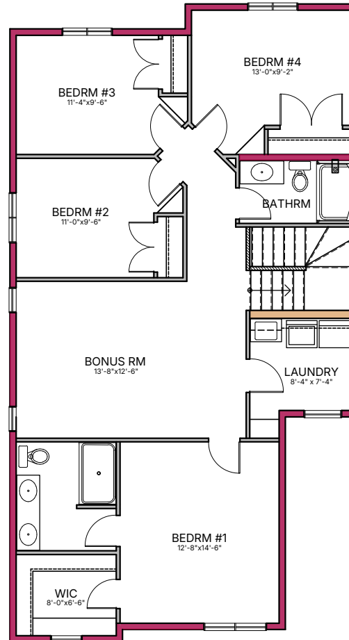
SECOND FLOOR - 1220 sq.ft. OPEN AREA - 59 sq.ft.
