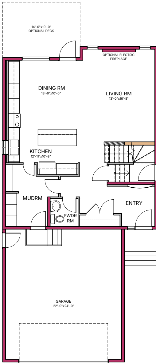
MAIN FLOOR - 896 sq.ft.
