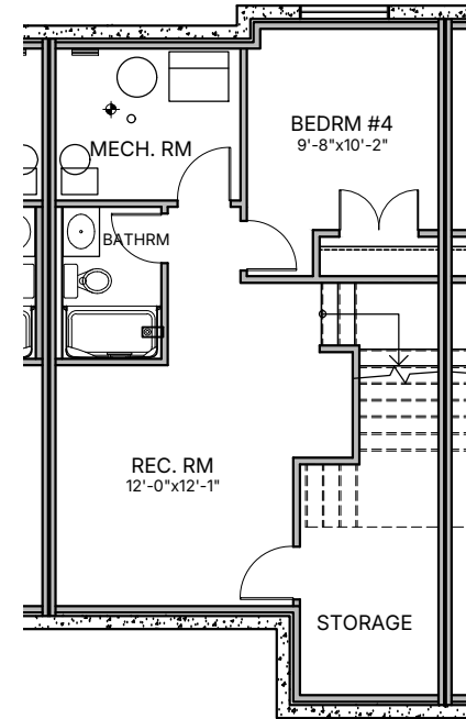
OPTIONAL BASEMENT LAYOUT - 660-802 sq.ft.
