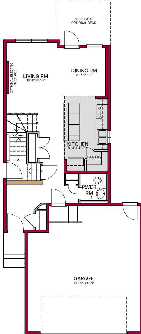
MAIN FLOOR - 653 sq.ft.
