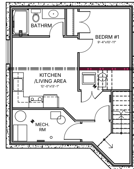
OPTIONAL BASEMENT SUITE LAYOUT - 674 sq.ft.
