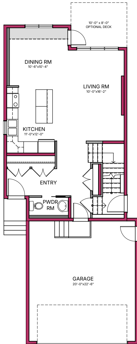
MAIN FLOOR - 714 sq.ft.
